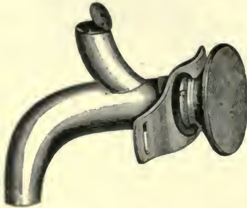
FIG. 881.—Gussenbauer's artificial larynx.
